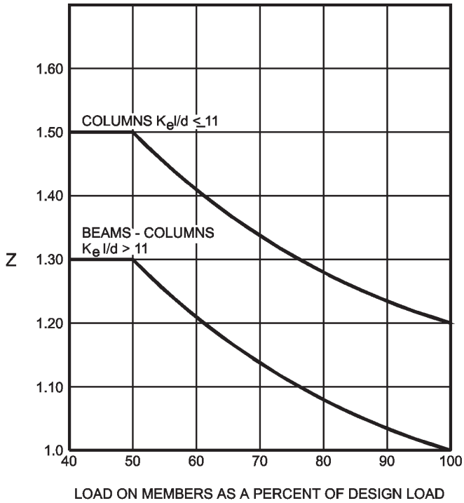
FIGURE 721.6.3(1) LOAD FIGURE
