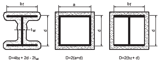
FIGURE 721.5.1(1) DETERMINATION OF THE HEATED PERIMETER OF STRUCTURAL STEEL COLUMNS
