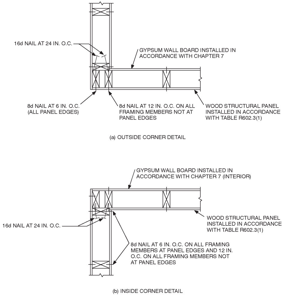
FIGURE R602.10.5(1) EXTERIOR CORNER FRAMING
