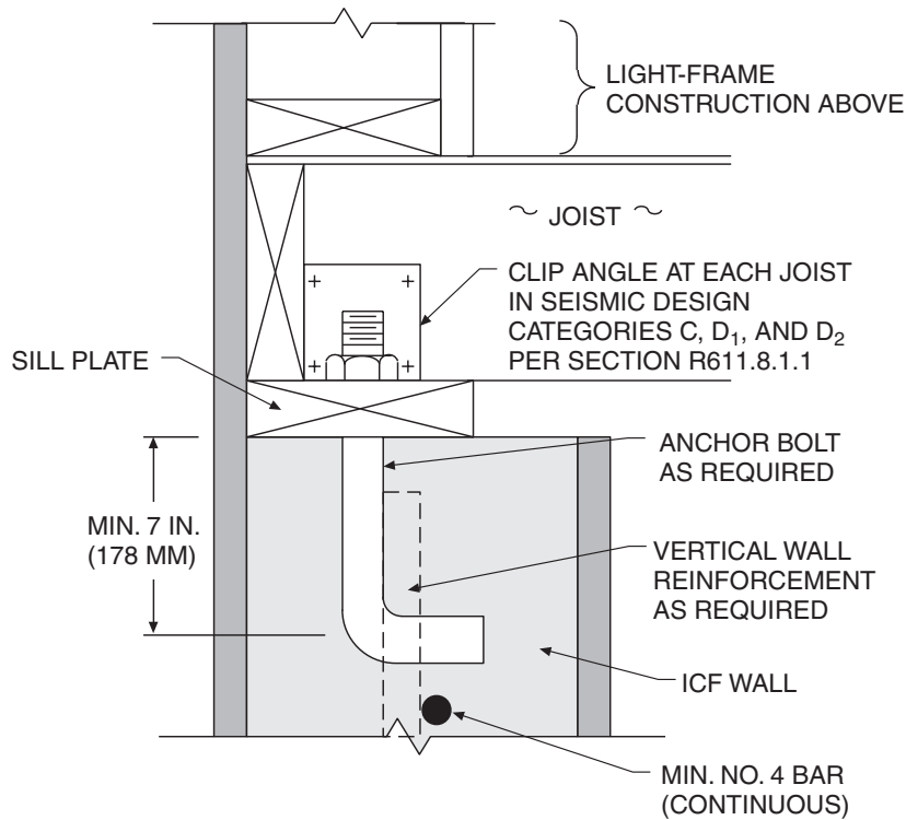
FIGURE R611.8(1) SECTION CUT THROUGH FLAT WALL OR VERTICAL CORE
