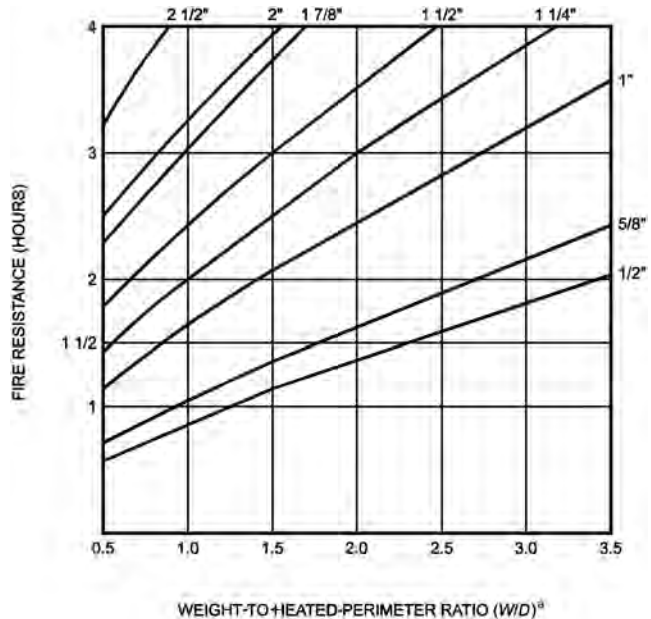
FIGURE 721.5.1(4) FIRE RESISTANCE OF STRUCTURAL STEEL COLUMNS PROTECTED WITH VARIOUS THICKNESSES OF TYPE X GYPHUM WALLBOARD
