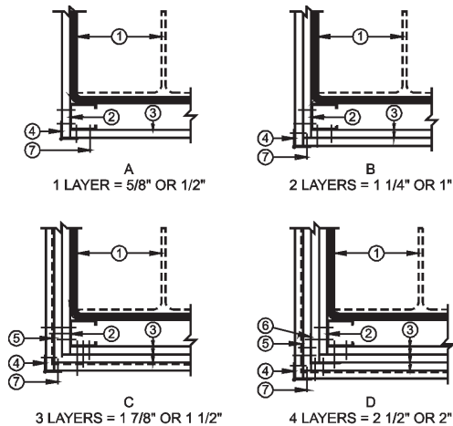
FIGURE 721.5.1(3) GYPHUM WALLBOARD PROTECTED STRUCTURAL STEEL COLUMNS WITH STEEL STUD/SCREW ATTACHMENT SYSTEM
