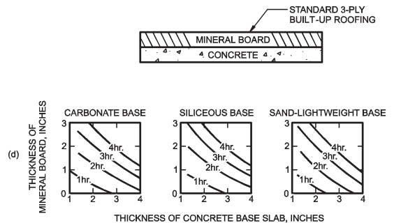
FIGURE 721.2.2.3(1) FIRE-RESISTANCE RATINGS FOR CONCRETE ROOF ASSEMBLIES
