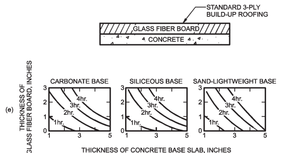
FIGURE 721.2.2.3(2) FIRE-RESISTANCE RATINGS FOR CONCRETE ROOF ASSEMBLIES
