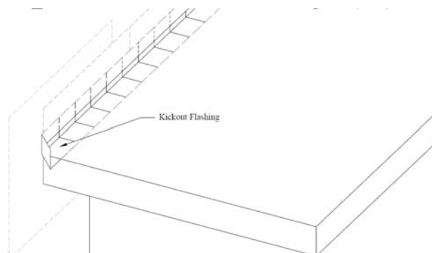
FIGURE R703.8(1) KICK-OUT FLASHING
