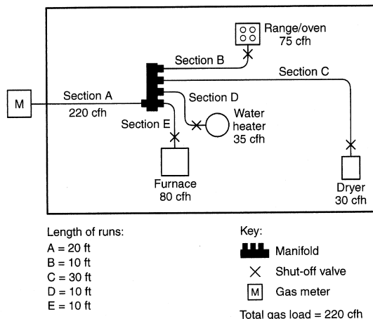
FIGURE C-A.6.3 PIPING PLAN SHOWING A COPPER TUBING SYSTEM
