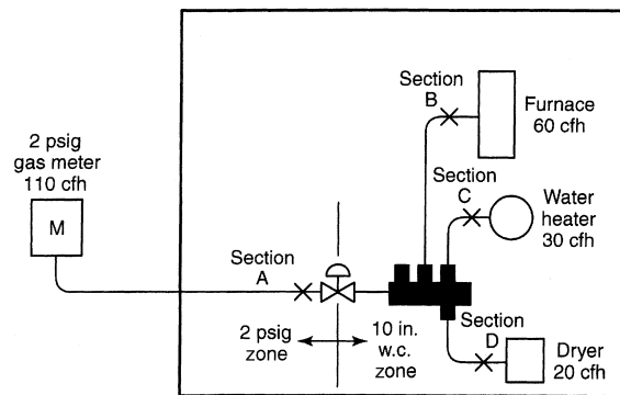
Length of runs: A = 100 ft B = 15 ft C = 10 ft D = 25 ft Key: Manifold Shut-off valve Pressure regulator Gas meter
