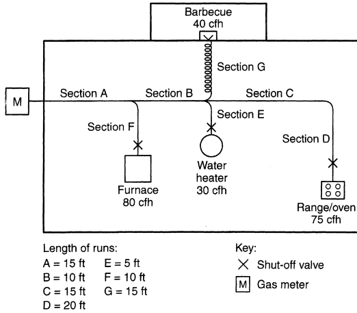
FIGURE C-A.6.4 PIPING PLAN SHOWING A MODIFICATION TO EXISTING PIPING SYSTEM
