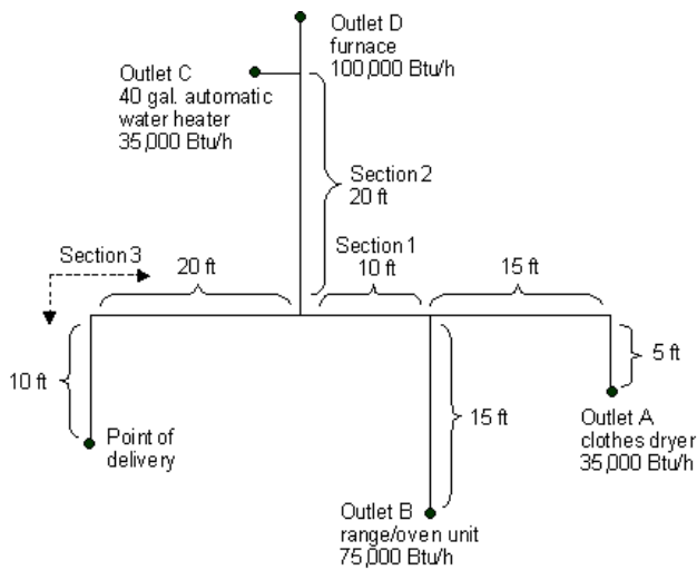
FIGURE C-A.6.1 PIPING PLAN SHOWING A STEEL PIPING SYSTEM
