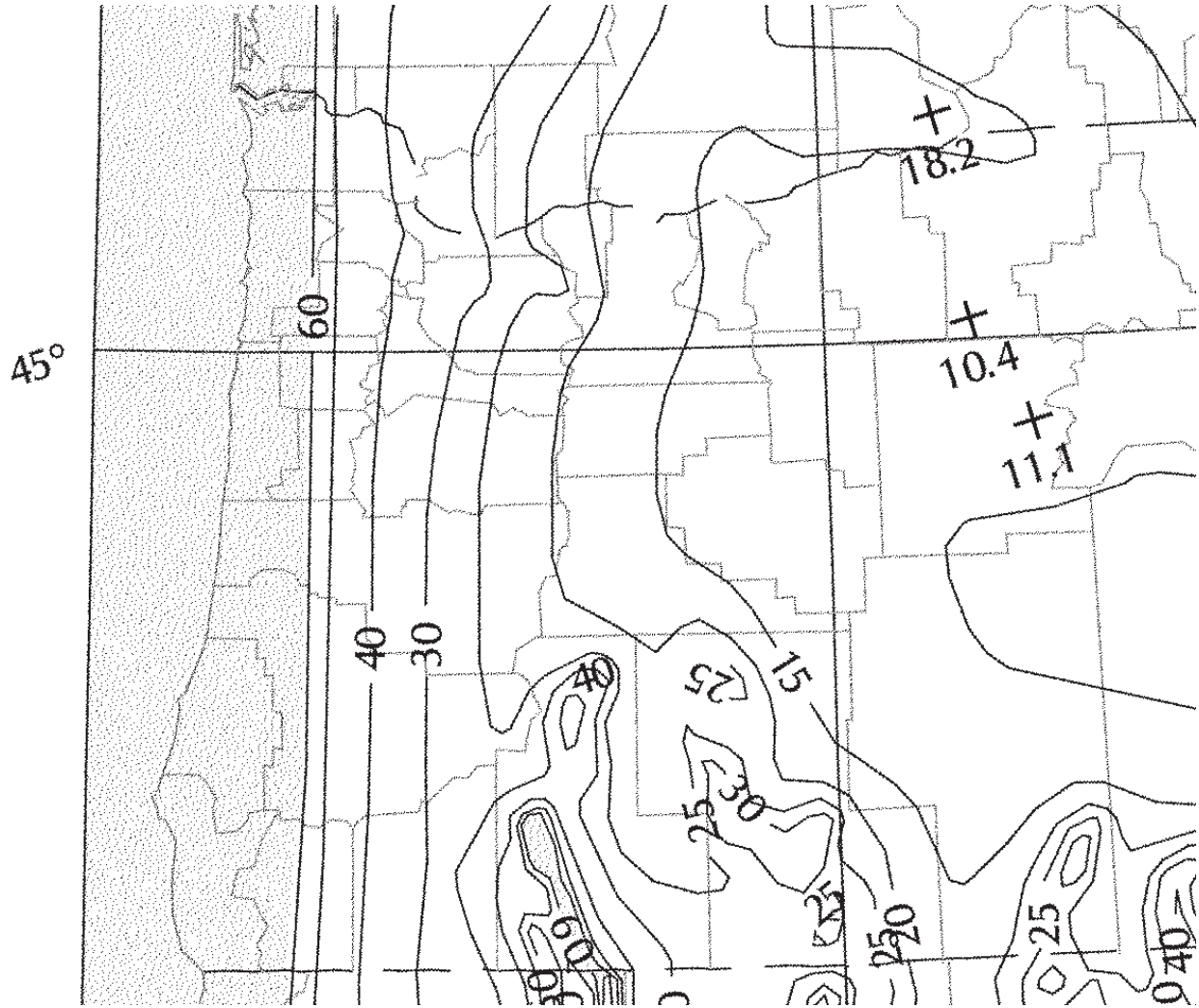
FIGURE 1615(2) MAXIMUM CONSIDERED EARTHQUAKE GROUND MOTION FOR OREGON STATE OF 1.0 SEC SPECTRAL RESPONSE ACCELERATION (5 PERCENT OF CRITICAL DAMPING), SITE CLASS B
