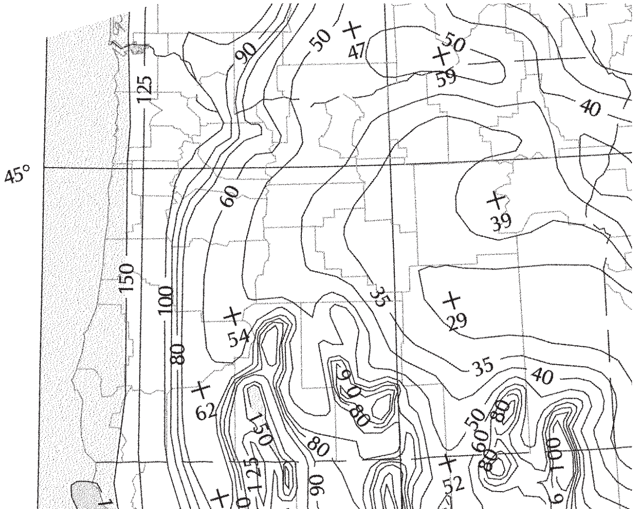
FIGURE 1615(1) MAXIMUM CONSIDERED EARTHQUAKE GROUND MOTION FOR OREGON STATE OF 0.2 SEC SPECTRAL RESPONSE ACCELERATION (5 PERCENT OF CRITICAL DAMPING), SITE CLASS B
