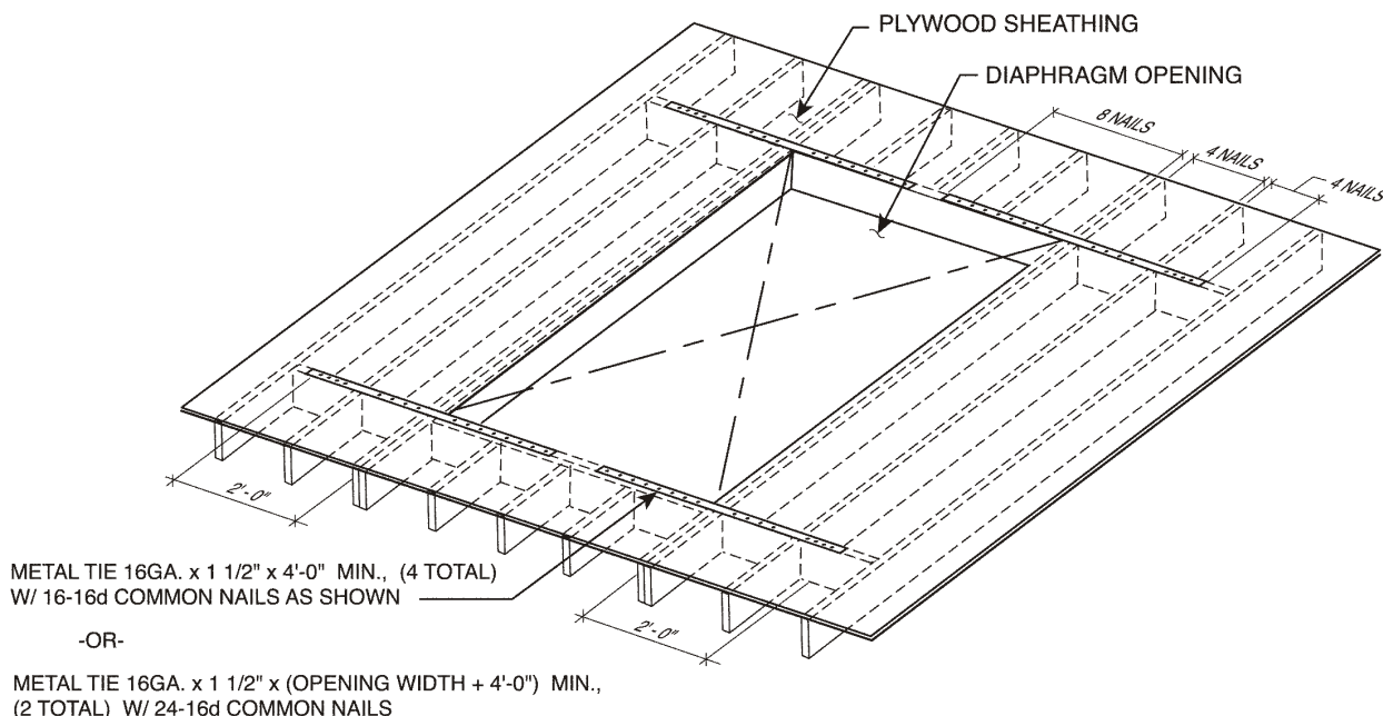
FIGURE 2308.11.3.3 OPENINGS IN HORIZONTAL DIAPHRAGMS
