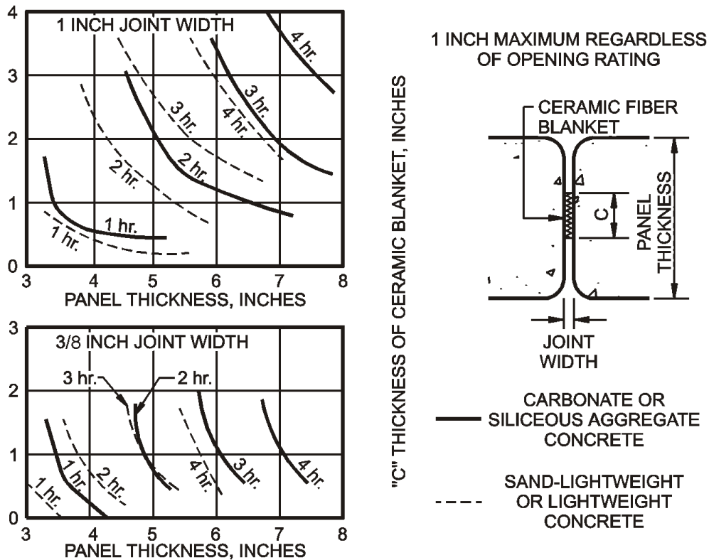
FIGURE 721.2.1.3.1 CERAMIC FIBER JOINT PROTECTION
