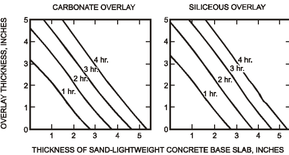
FIGURE 721.2.2.2 FIRE-RESISTANCE RATINGS FOR TWO-COURSE CONCRETE FLOORS
