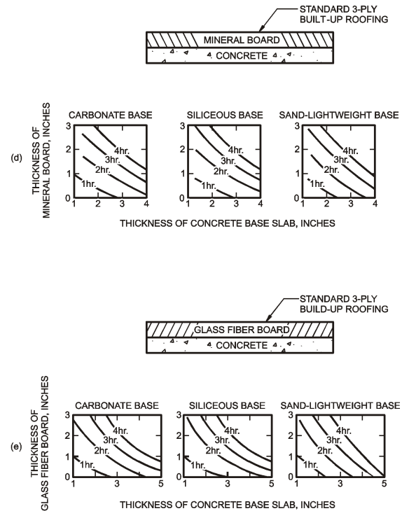
FIGURE 721.2.2.3(2) FIRE-RESISTANCE RATINGS CONCRETE ROOF ASSEMBLIES
