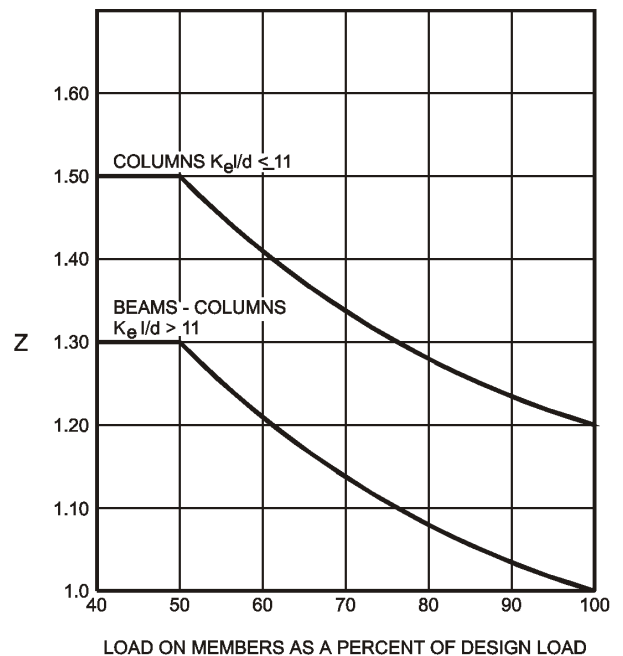
FIGURE 721.6.3(1) LOAD FIGURE
